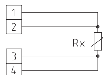
1x four-wire connection
